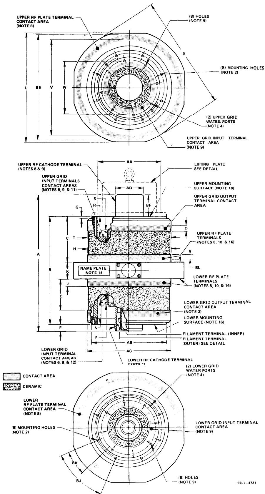
Figure 4 - Dimensional Outline
